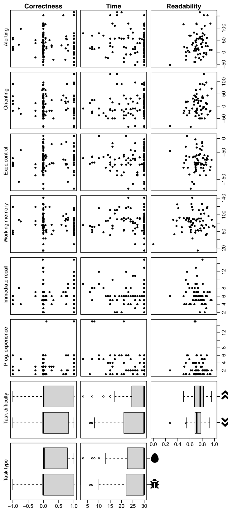
Fig. 3: Relationships between the independent variables (y axis) and dependent variables (x axis). We use scatter plots for continuous variables and box plots for binary ones. \bullet and \blacklozenge indicate task type ( bug fixing and feature implementation ), while \blacktriangleleft and \blacktriangleright indicate the task difficulty ( easy and hard ).
